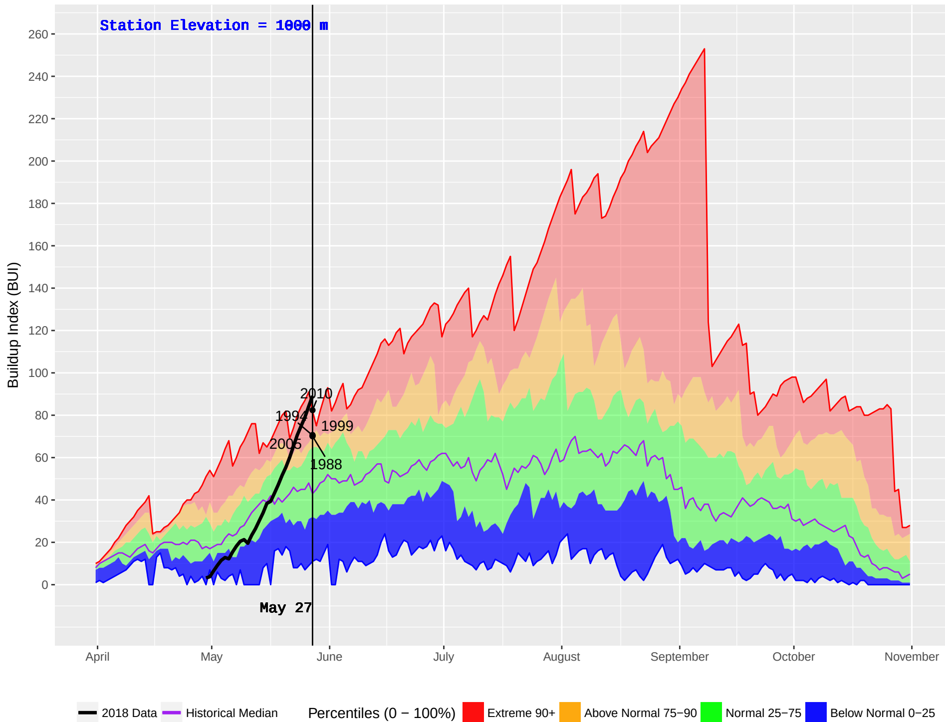
SUCCOUR CREEK (374) : Historical (1986–2016) and Current (2018) Noon Buildup Index (BUI)
