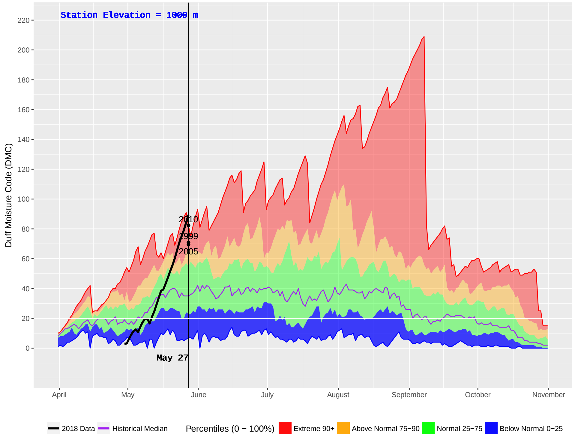
SUCCOUR CREEK (374) : Historical (1986–2016) and Current (2018) Noon Duff Moisture Code (DMC)
